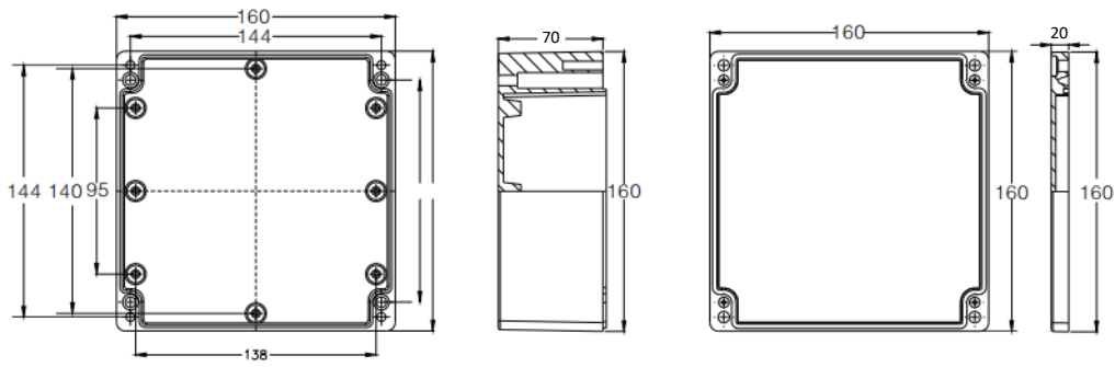
CRADYBOX-AL-160X160X90 - 0186005
