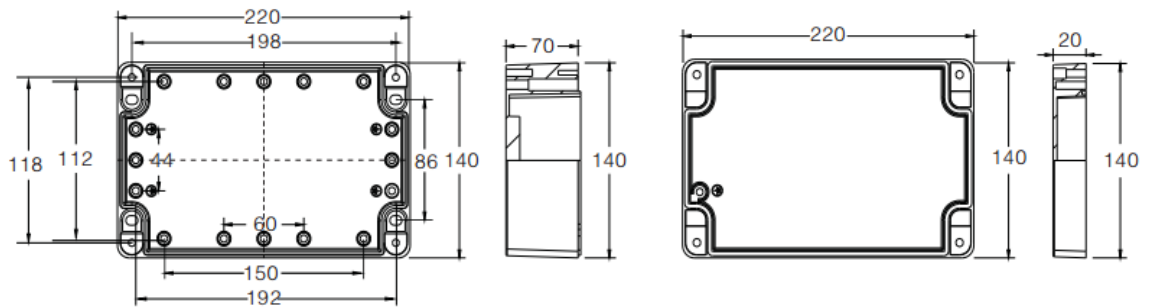
CRADYBOX-AL-220X140X90 - 0186006
