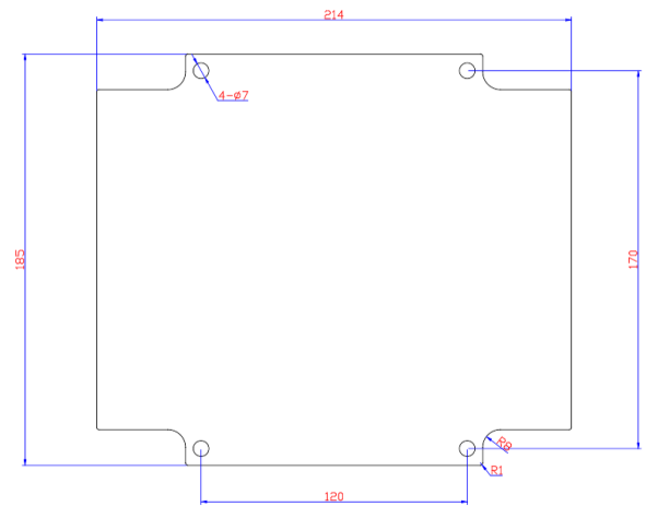
PM-CRADYBOX-AL-320X230X120 - 0186108
