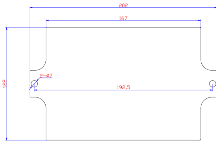
PM-CRADYBOX-AL-320X230X120 - 0186108
