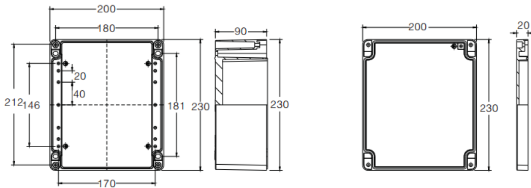
CRADYBOX-AL-230X200X110 - 0186007
